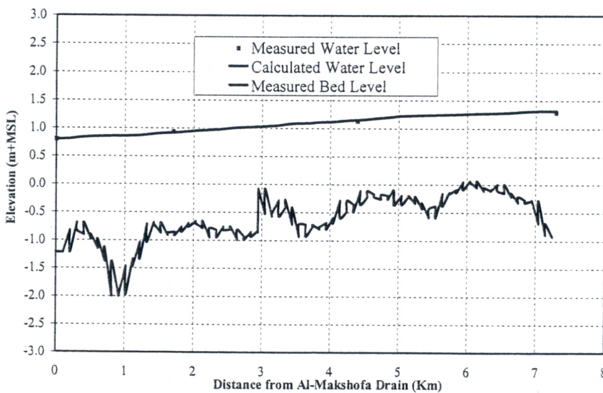
Fig. 4: Model calibration
