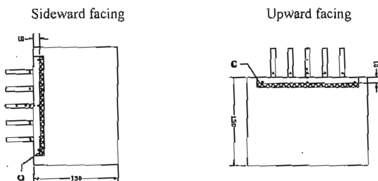
Fig. 2 Heat sink orientations
