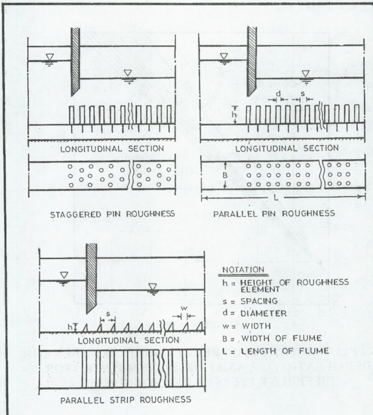
FIG.1 – ARRANGEMENT OF ROUGHNESS ELEMENTS
