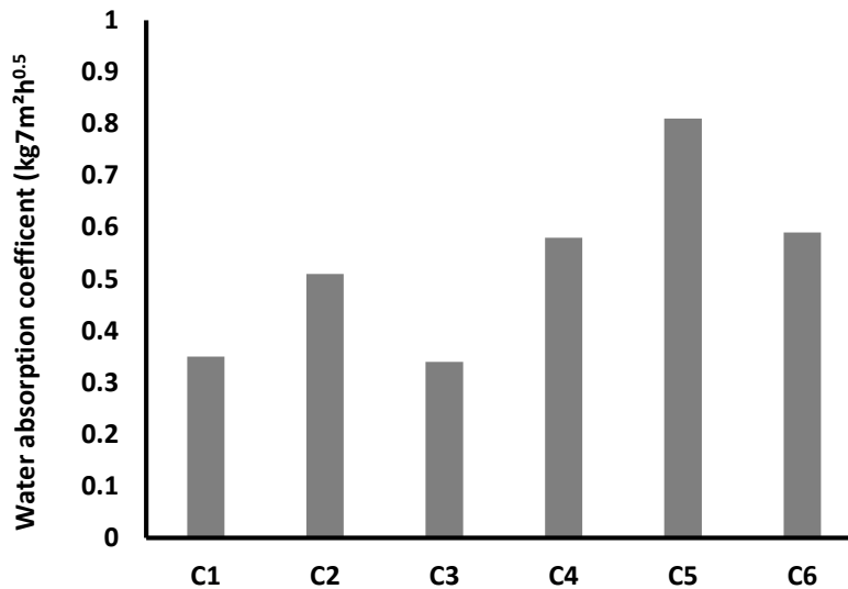
Fig.9: Water absorption coefficient o LWC mixes
