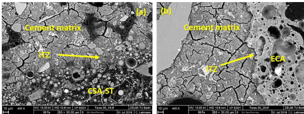
Fig. 10. Scanning electron microscopy of transition zone of concrete at age of 28 days: (a) treated aggregates, (b) Liapor
