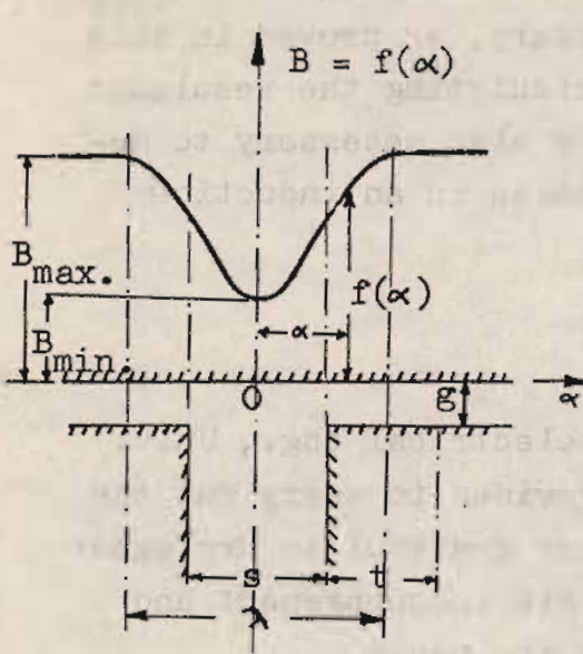
Fig. (1) Flux density variation due to slotting.
