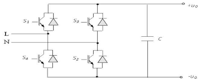
Fig. 13 DC/AC H-bridge converter
