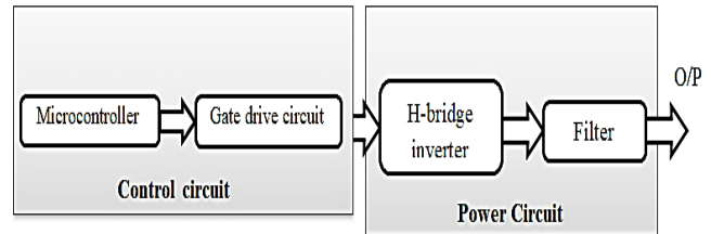
Fig. 12 Block diagram of the complete designed inverter
