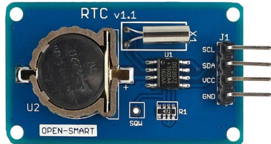
Fig.7. Real time clock circuit used in the system
